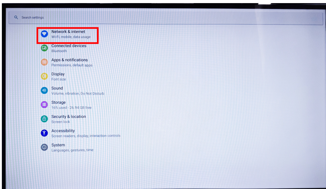
Settings screen
